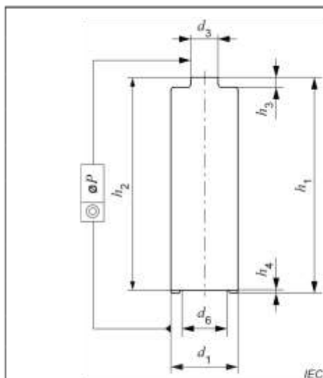
Dimensional drawing: LR6, FR14505, R6P, R6S
